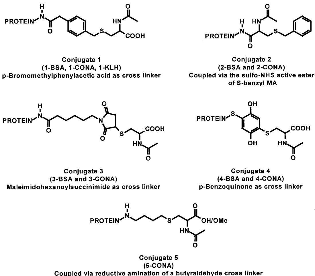
Figure 1. Structures of hapten–protein conjugates used as the immunogen (conjugate 1) and as coating antigens (conjugates 2–5). Conjugates 3-CONA and 5-CONA were selected for the final coating antigens.
